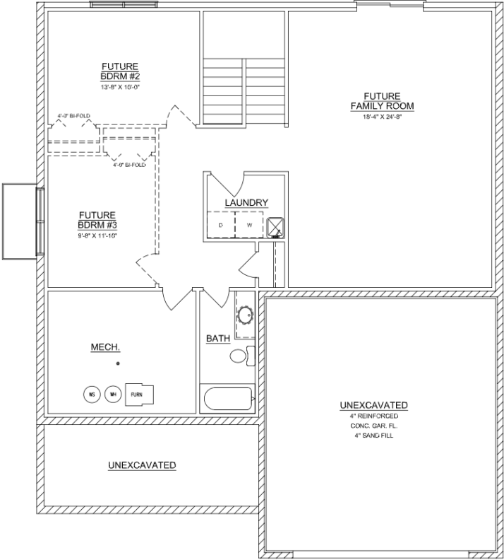
1 BASEMENT & FOUNDATION PLAN SCALE: 1/4" = 1'-0"
