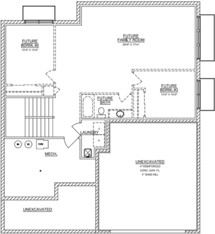
1 BASEMENT & FOUNDATION PLAN SCALE: 1/4" = 1'-0"
